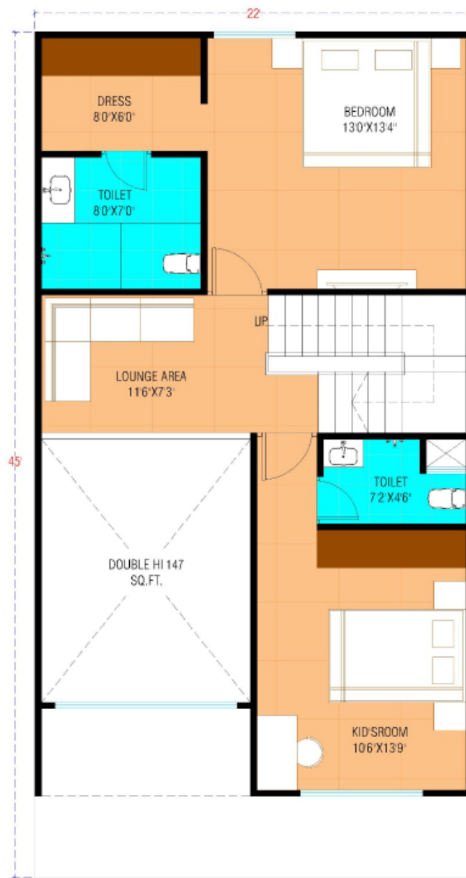
MEZZANINE FLOOR PLAN
